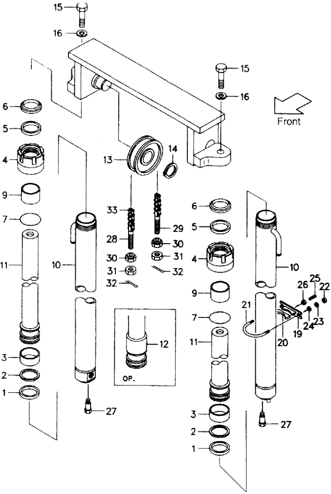
Fig.48 LIFT CYLINDER [VM41A]
