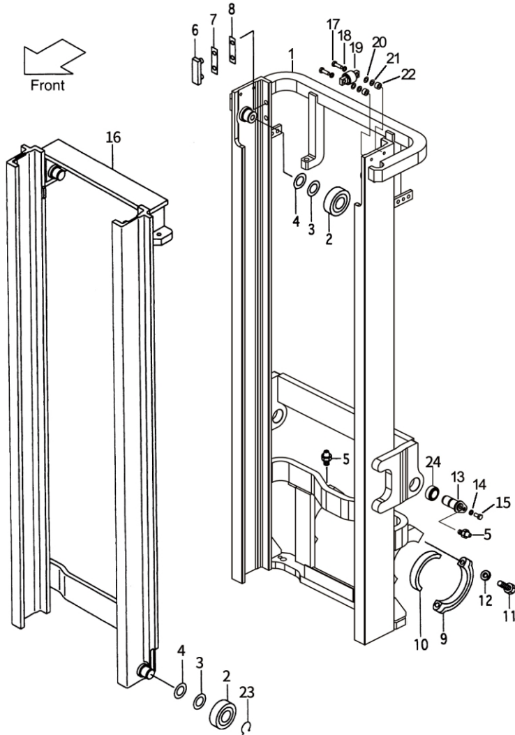
Fig.42 MAST [VM21A]
