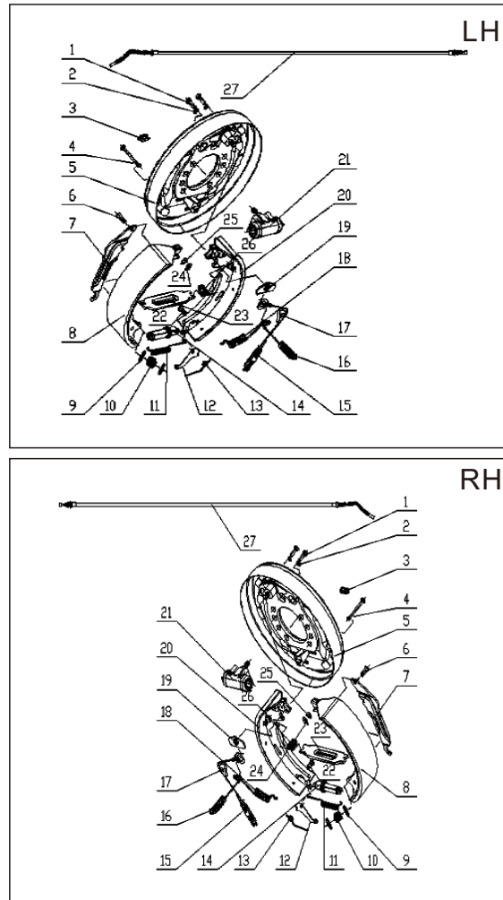
Fig.11 DRIVE AXLE ( 3-3.5 )
