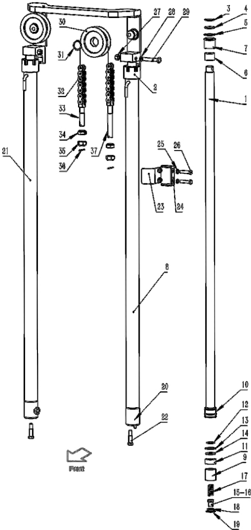
Fig.54 LIFT CYLINDER (REAR) [VF3M31A]
