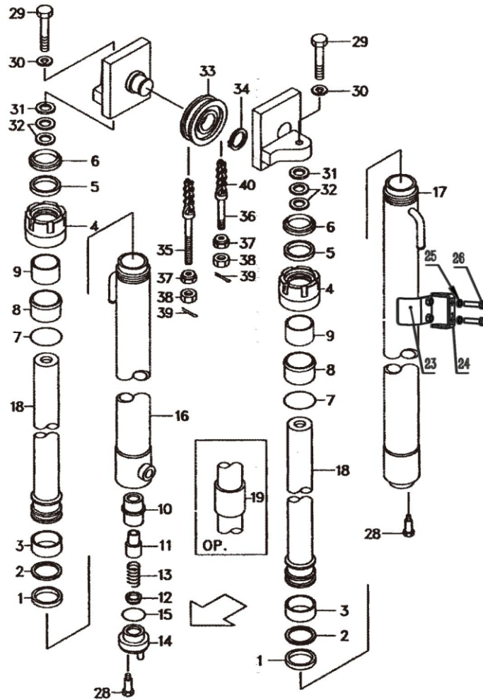
Fig.55 LIFT CYLINDER (REAR) [VF36E] [VF41E]
