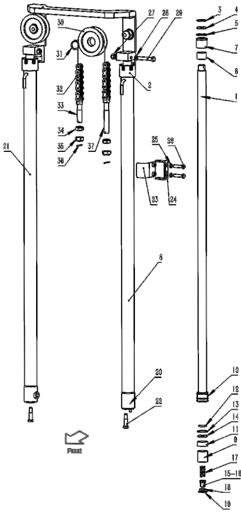
Fig.69 LIFT CYLINDER (REAR) [VF5M31A]
