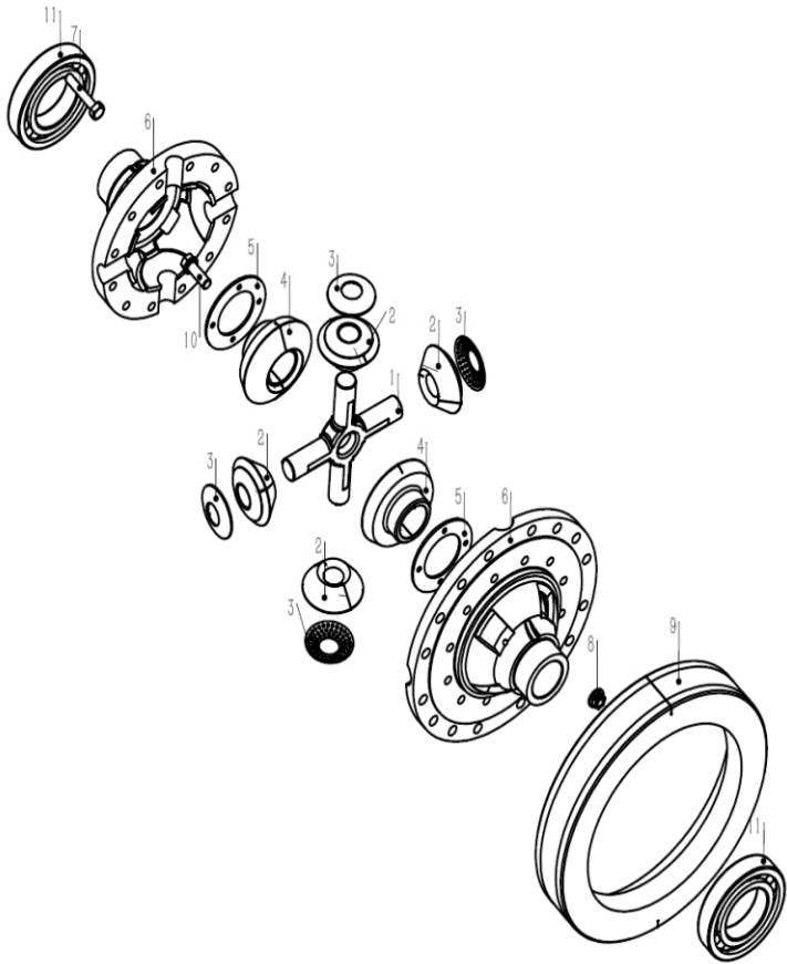
Fig.17 REDUCTION & DIFFERENTIAL
