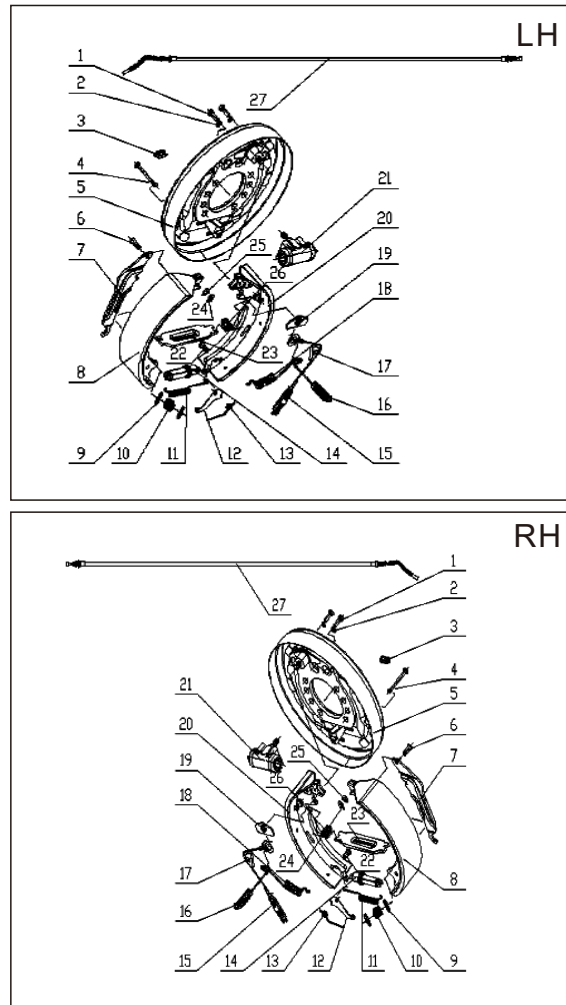
Fig.18 WHEEL BRAKE ( 3-3.5 )
