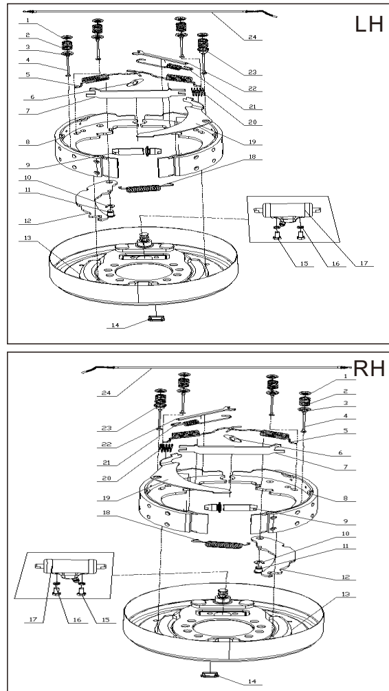
Fig.18 WHEEL BRAKE ( AQ2-2.5 )
