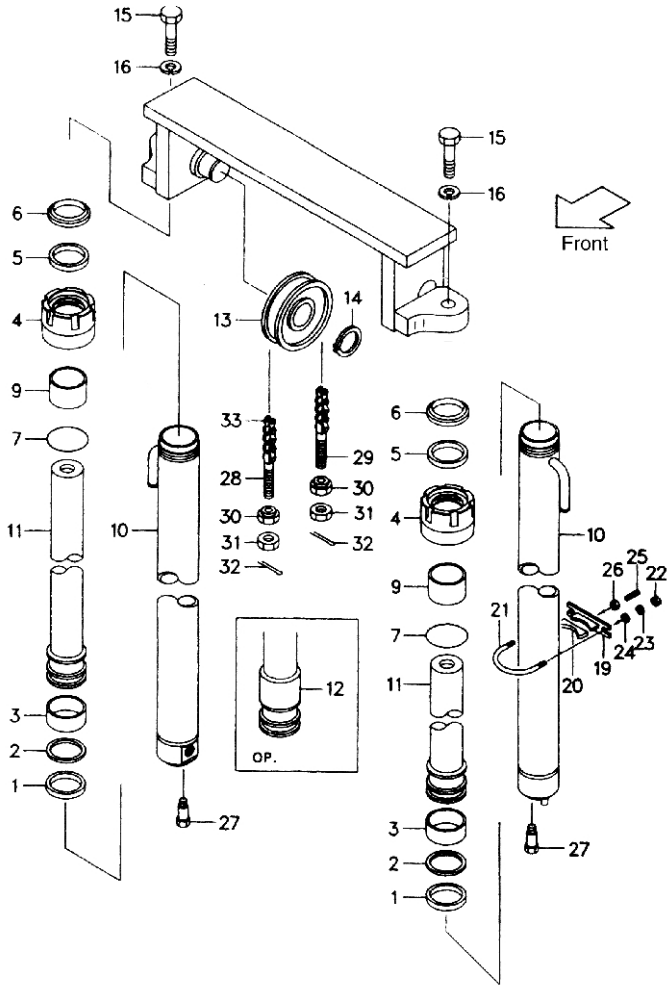
LIFT CYLINDER [VM21A]
