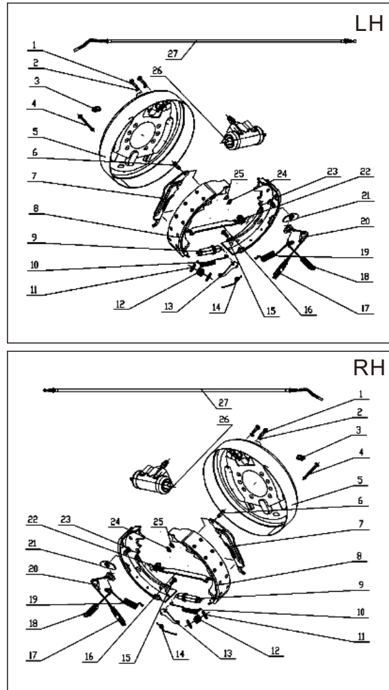
Fig.18 WHEEL BRAKE ( 2-2.5 )
