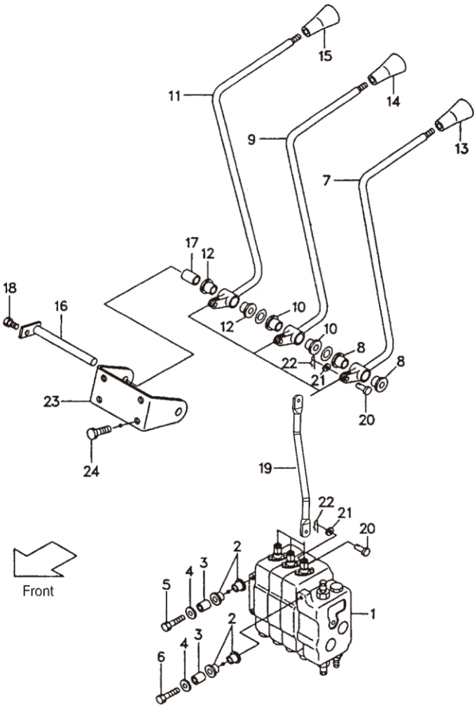
Fig.37 VALVE CONTROL LINKAGE (3SV)
