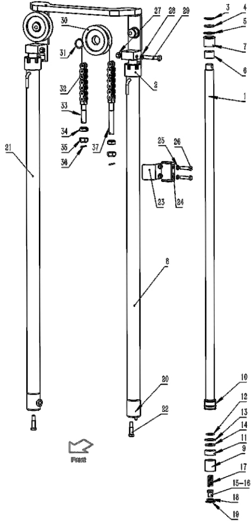
Fig.69 LIFT CYLINDER (REAR) [VF31A]
