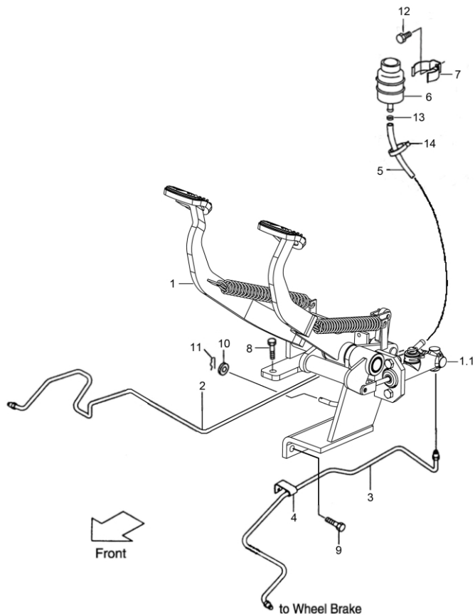
Fig.25 BRAKE PEDAL
